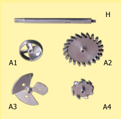
shaft and mixer heads:
